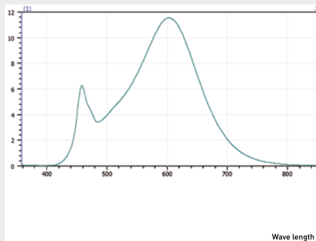
Spectral intensity
