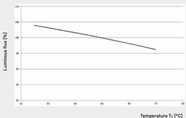
Relative luminous flux based on Tc
