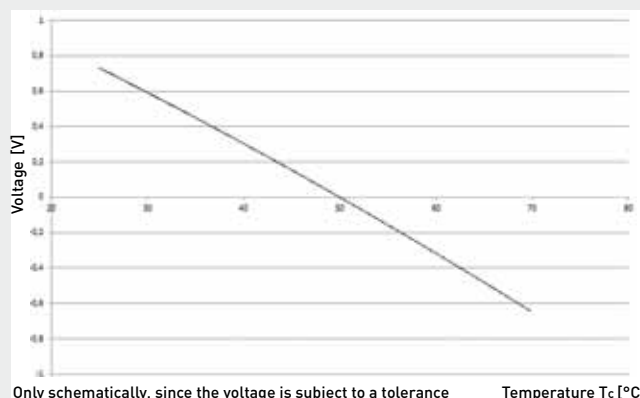
Voltage / temperature
