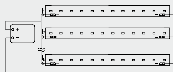
Parallel connection
