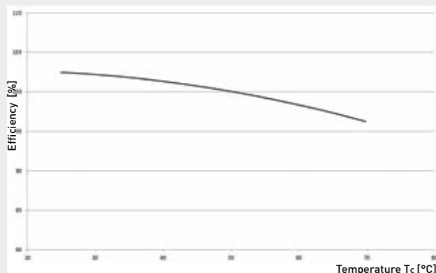
Efficiency / temperature
