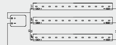
Parallel connection
