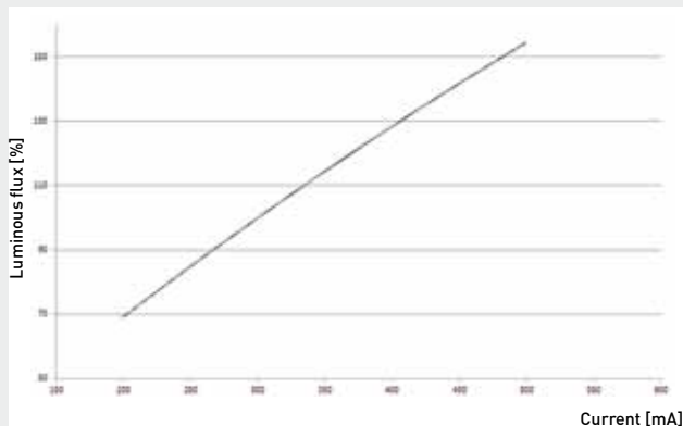
Relative luminous flux based on operational current
