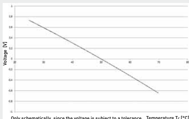
Voltage / temperature
