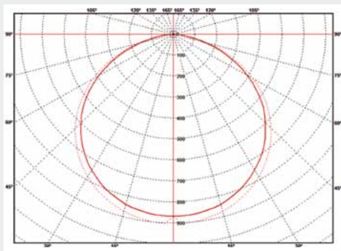
Light distribution
