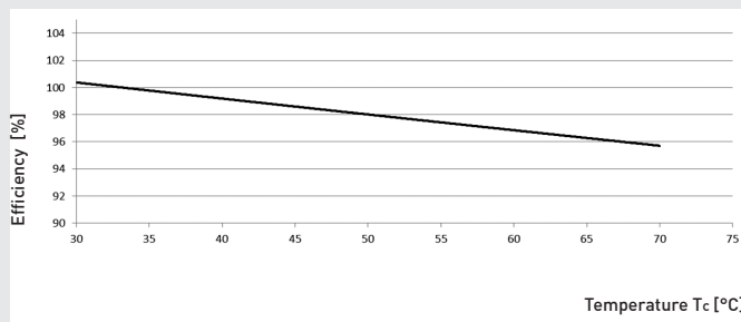
Efficiency / temperature
