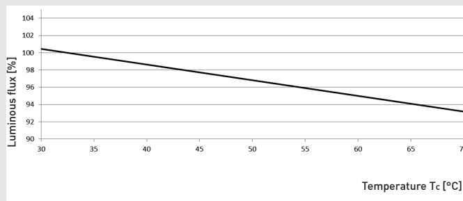
Relative luminous flux based on Tc
